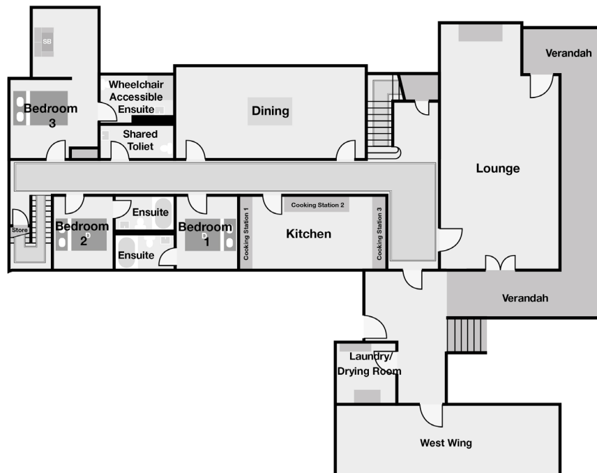
Caves House 1917 Section - Ground Floor
